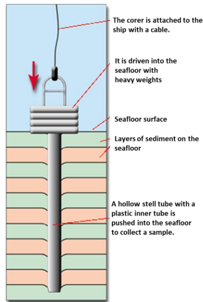
Figure 5.8 Example of a corer. Source: British Ocean Sediment Core Research Facility.
