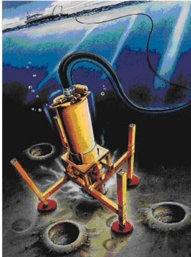
Figure 5.9 An artists impression of a sampling drill tool with a drill bit footprint of 3 m 2 .
