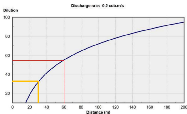
Figure 5.16. Long shore achievable dilutions versus distance calculated from False Bay field experiments (CSIR 1992). Achievable dilutions at 60 m and 30 m are shown in red in yellow respectively.
