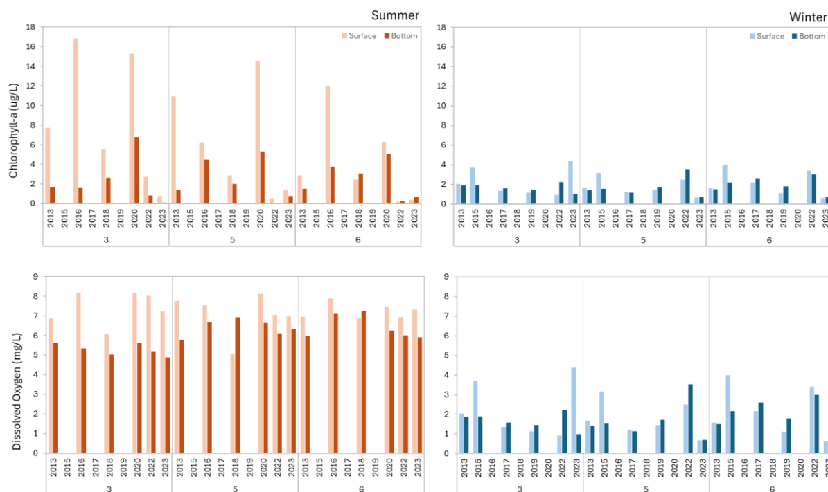
Figure 3.13 (cont.). Physico-chemical parameters for summer and winter surveys at the surface and bottom of the water column at three stations: in the middle of the estuary (3), at the mouth (5) and just out to sea beyond the breakwater (6). Data from (CSIR 2014, 2016, 2018, 2020, 2023c a).
