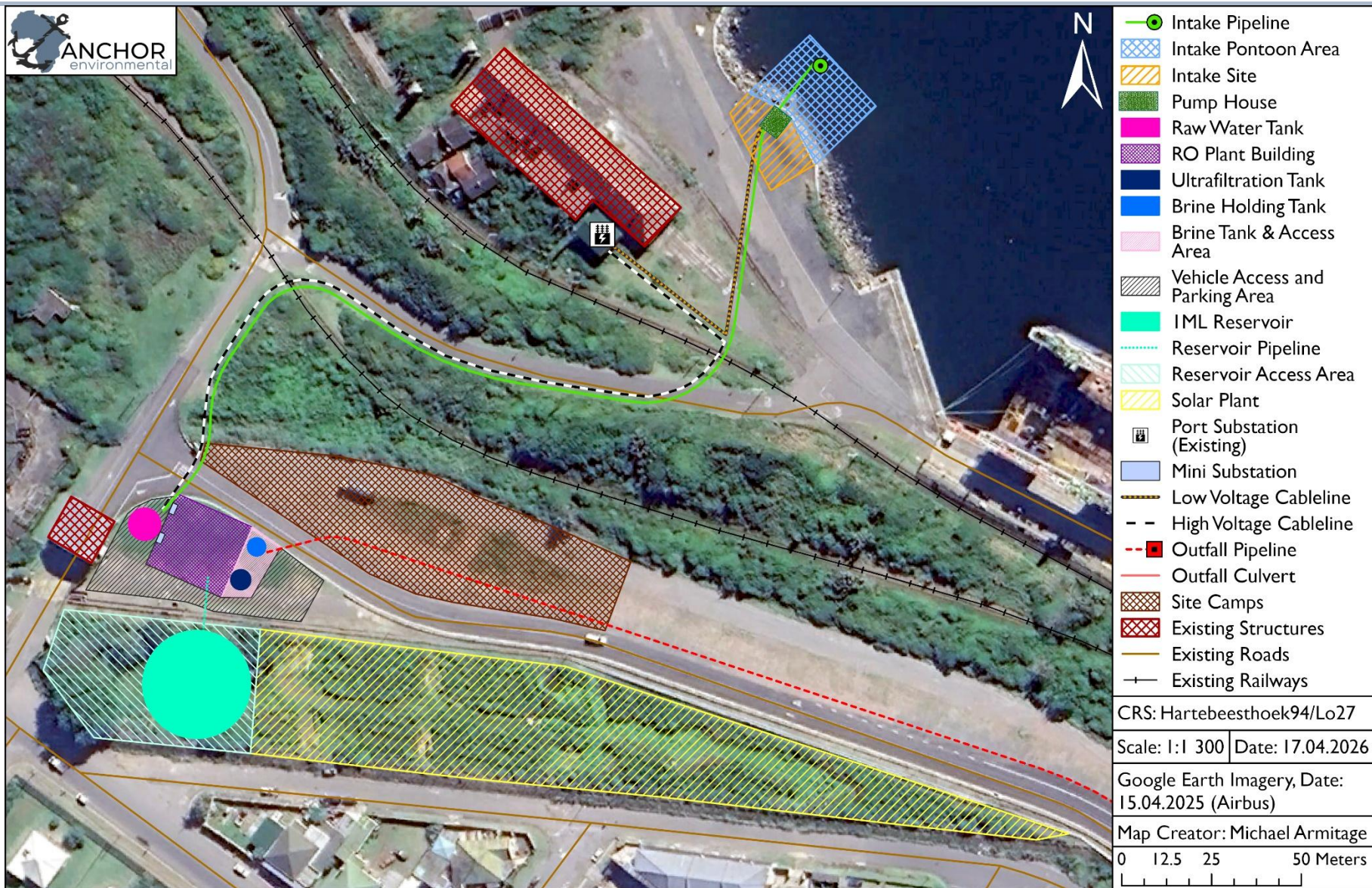
Figure 1.4. The proposed intake, RO Plant, Solar Plant, and all supporting infrastructure.
